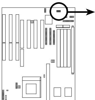
PS/2 Mouse Module Connector
