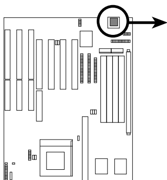
Keyboard Connector (5-pin female)
