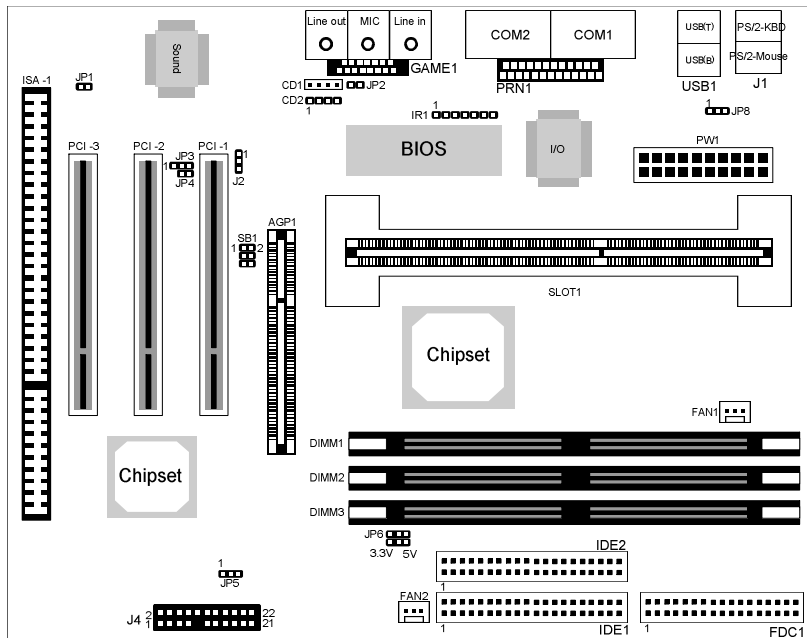
Figure 2-1. Mainboard Component locations
