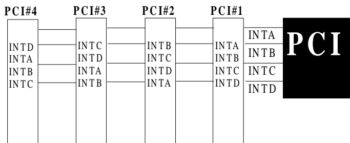
Figure 7: The Combination of PCI INT#lines
