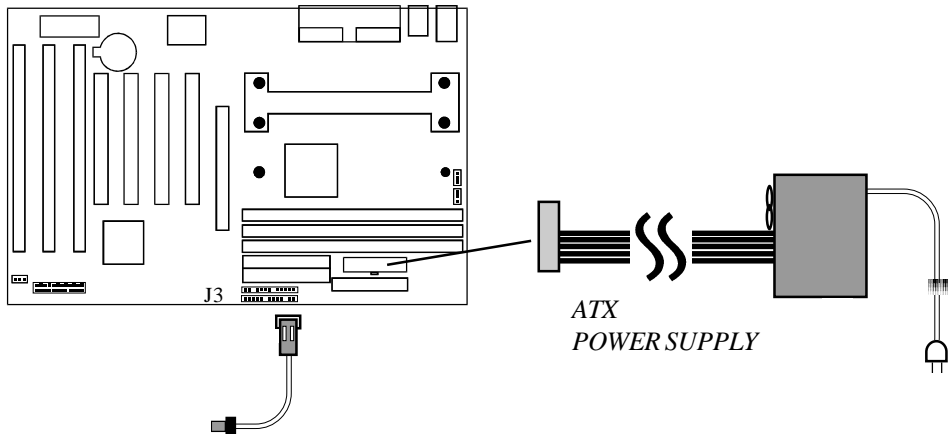
EP-61BXA-M Board Case (chassis) Power ON/OFF button
