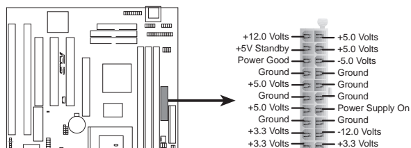
P5A-B ATX Power Connector
