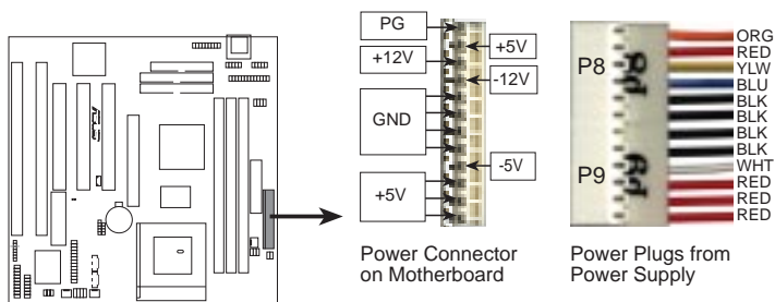
P5A-B AT Power Connector
