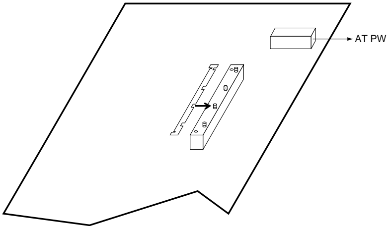
Top View of CPU Support Clip
