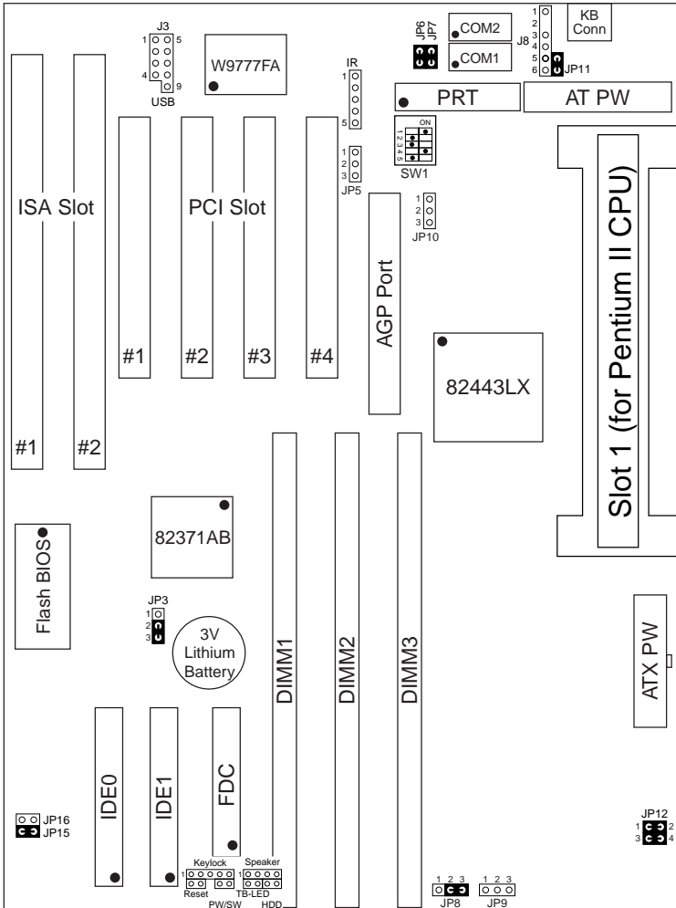
Figure 1-2. Mainboard Default Setting
