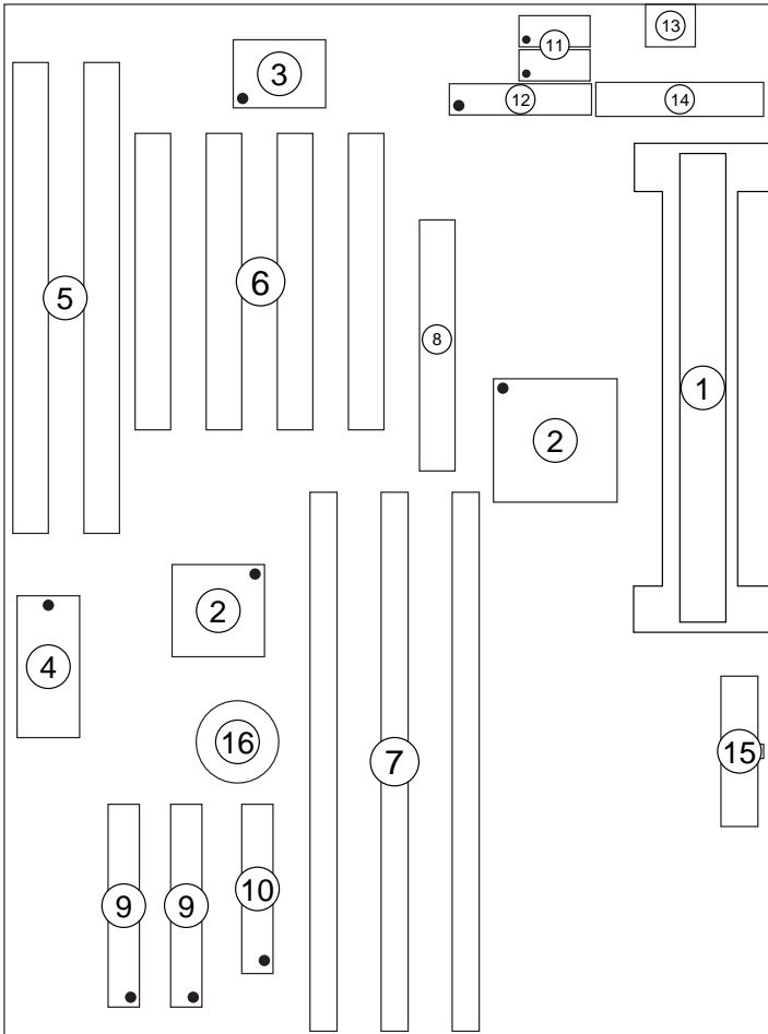
Figure 1-1. Mainboard Layout
